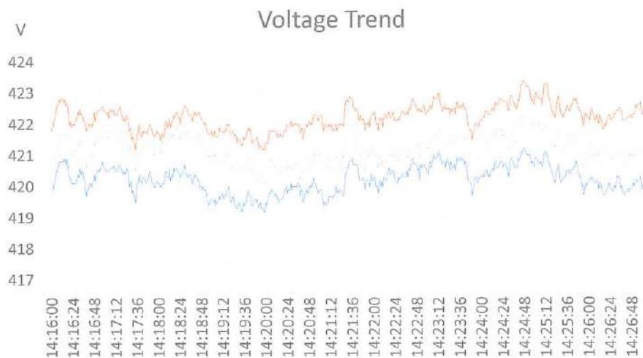
Figure 19-College of Management Voltage Profile
