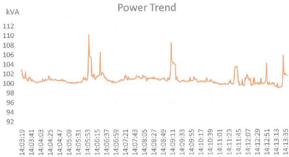
Figure 27-College of Pharmacy Power Consumption Profile – kVA
