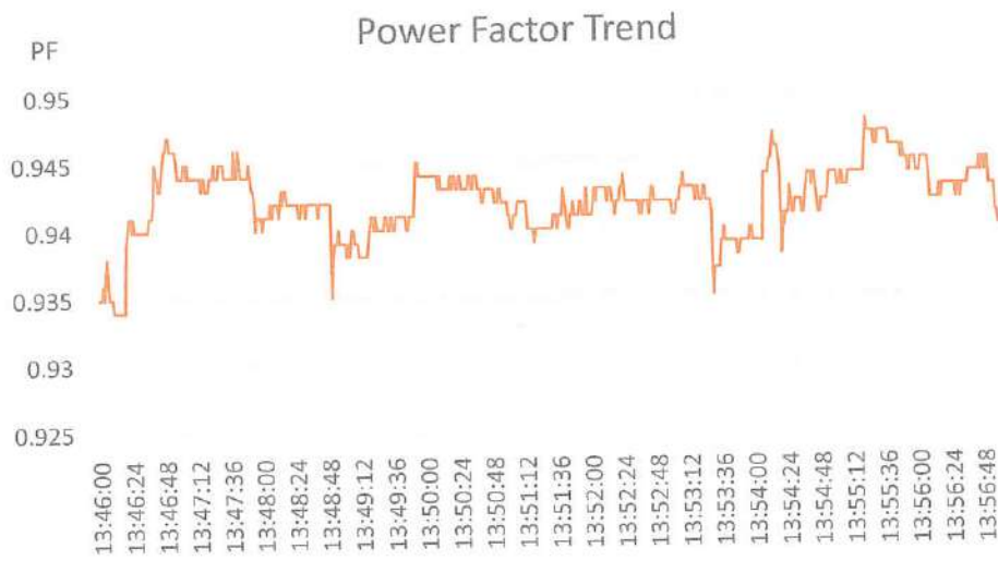
Figure 32- College of Polytechnic Power Factor Profile
