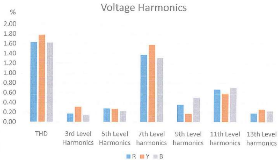
Figure 8-. Voltage Harmonics Profile – College of Pharmacy
