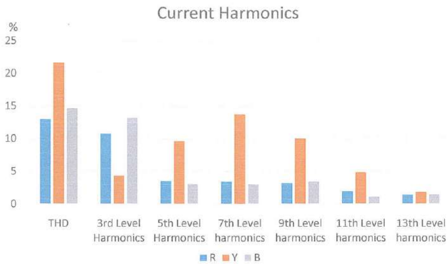
Figure 11- Current Harmonics – Management College
