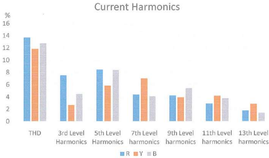
Figure 12- Current Harmonics – College of Pharmacy
