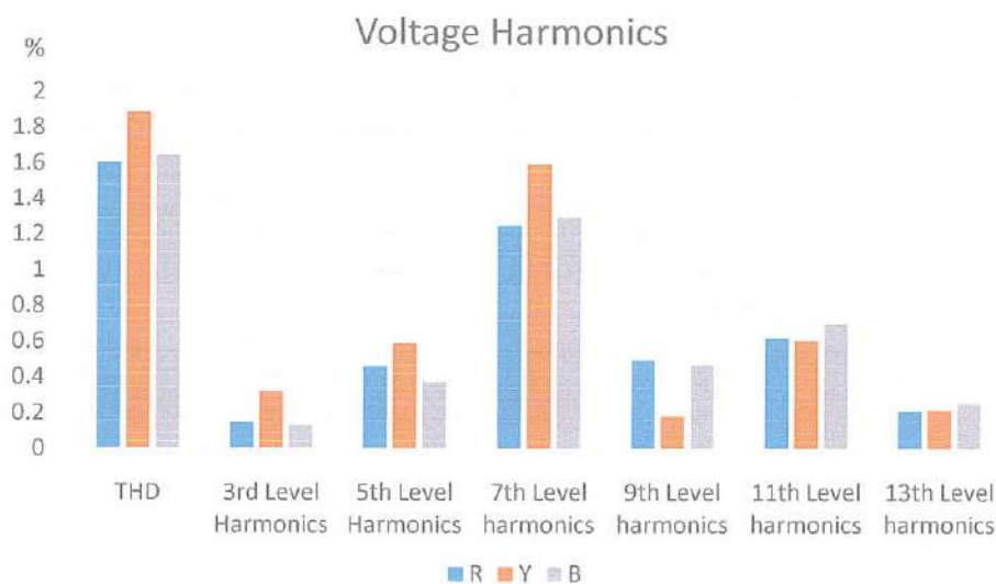
Figure -6. Voltage Harmonics Profile – Engineering College
