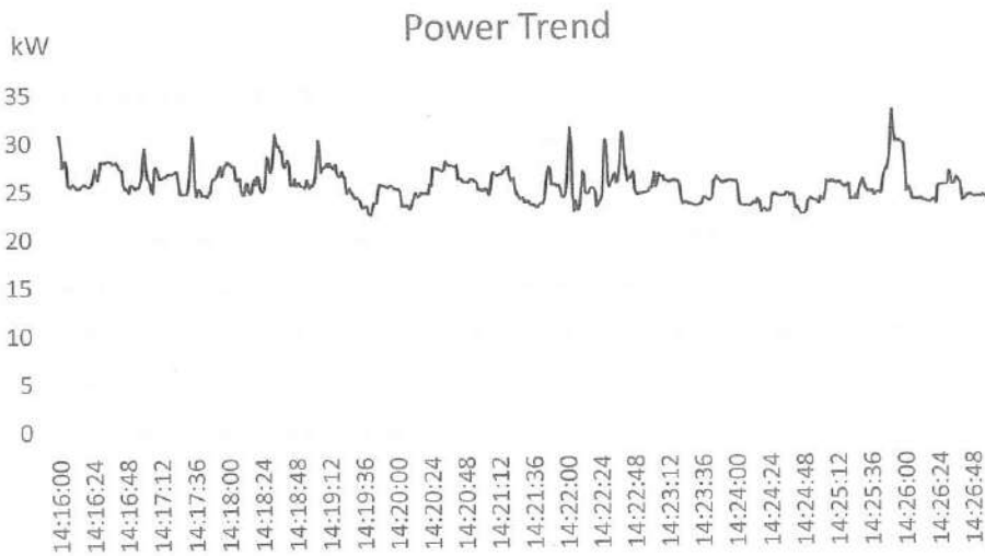
Figure 21- College of Management Power Consumption Profile – kW
