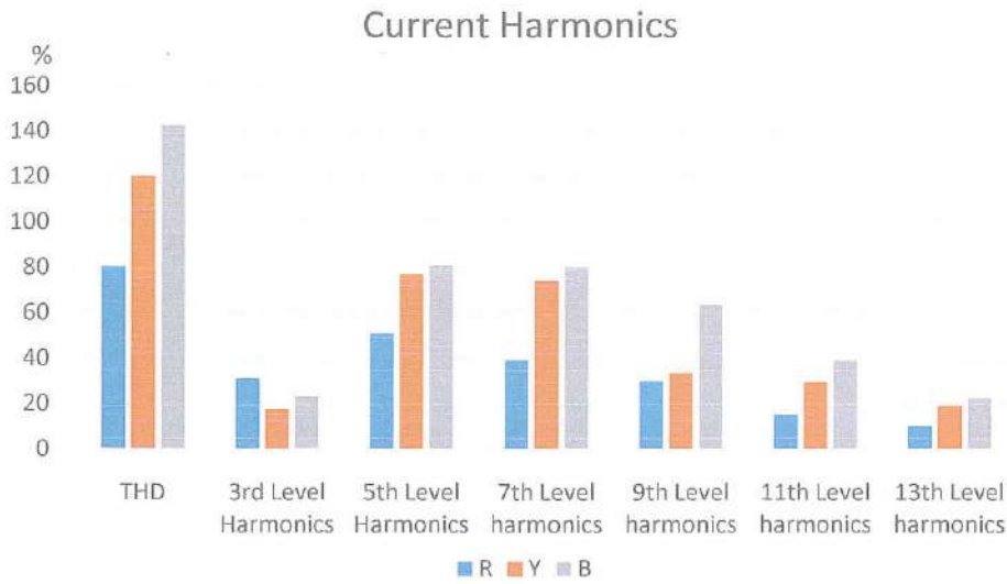
Figure 10- Current Harmonics– Engineering College
