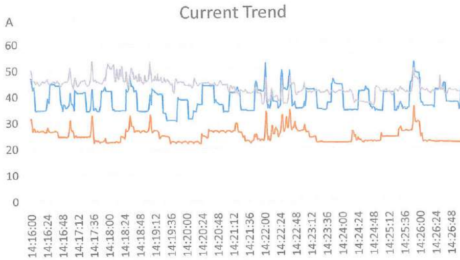
Figure 20- College of Management Current Profile
