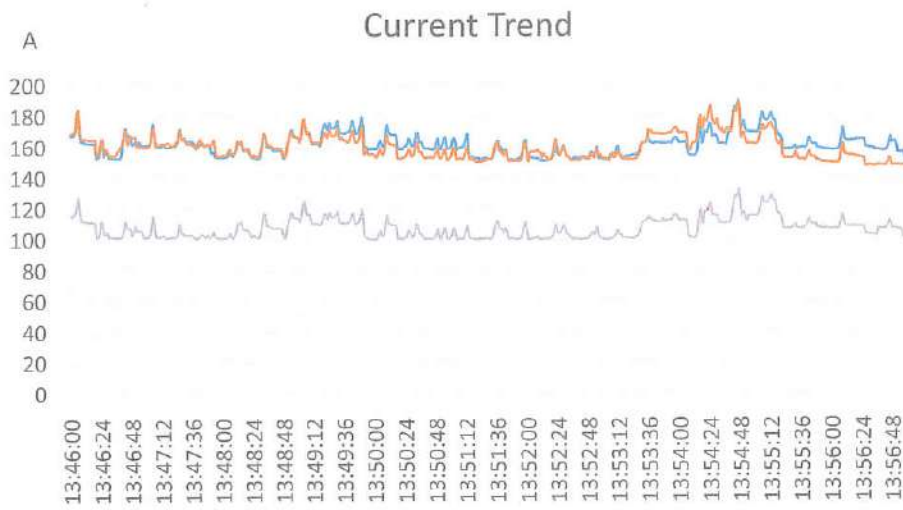
Figure 30- College of Polytechnic Current Profile
