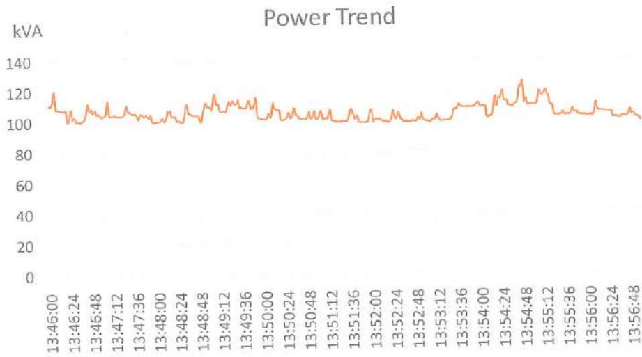
Figure 31-College of Polytechnic Power Consumption Profile – KVA
