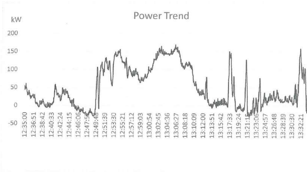
Figure 16- Engineering College Power Consumption Profile – kW
