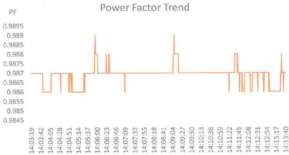
Figure 28- College of Pharmacy Power Factor Profile
