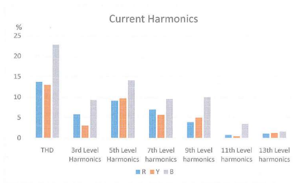
Figure 13- Current Harmonics – Polytechnic College
