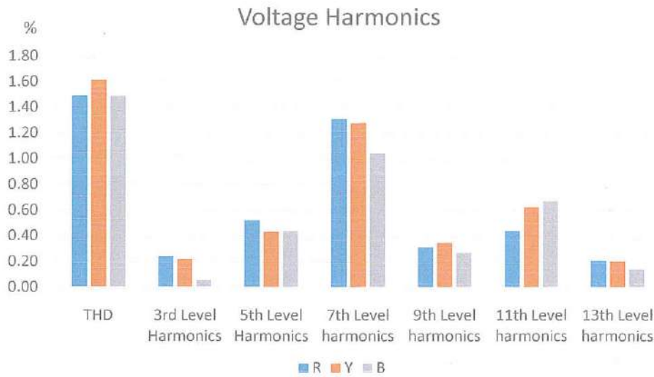
Figure 9- Voltage Harmonics Profile – Polytechnic College
