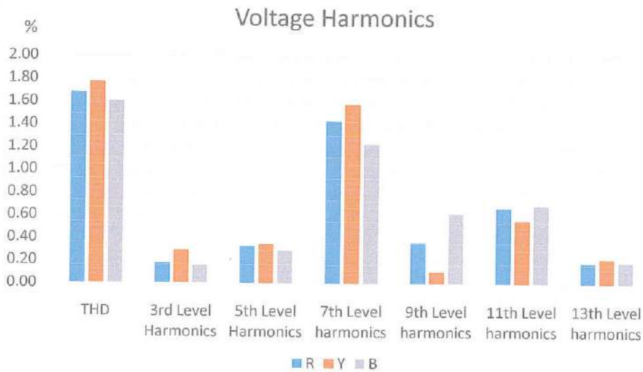
Figure7. Voltage Harmonics Profile – Management College
